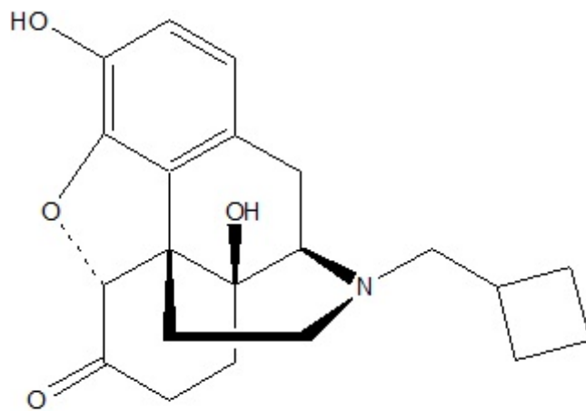
N-(cyclobutylmethyl)noroxymorphone
